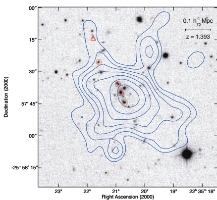
Figure 5: VLT ISAAC K-band image of XMMU J2235.3-2557 overlaid with X-ray contours (0.5 to 2 keV). Spectroscopically confirmed cluster members at 1.38 < z < 1.40 are marked in red and 1.37 < z < 1.38 in orange. Additional spectroscopically confirmed galaxy members lie outside this FOV. (Mullis et al. 2005).
