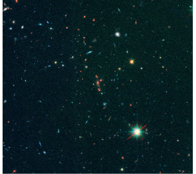
Fig. 1. A color image of XMMU J2235 obtained by combining the ACS F775W and F850LP and NICMOS F160W images ( North is up, East to the left ). The image shows a region of about 2 \times 2 arcmin 2 , corresponding to about 1 \times 1 Mpc 2 at the cluster redshift.
