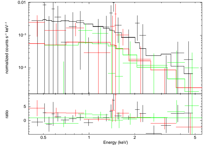
Fig. A.2. XMM-Newton X-ray spectrum of XMMU J1007 (EPIC-pn in black, EPIC-MOS in red and green). A thin thermal plasma model (the so-called MEKAL-model in the X-ray spectral fitting package XSPEC ) was fitted to the data. Fit optimisation was achieved by using the Cash-statistic with one count per bin (Krumpe et al. 2008). It does not, however, provide a goodness-of-fit statistic. The fit suggests a cluster temperature of T = 5.7 keV ( kT > 2.05 keV with 90% confidence). The temperature is not constrained towards high values. The bolometric X-ray luminosity of this model is L_X = 1.3 \times 10^{44} ergs s^{-1} .
