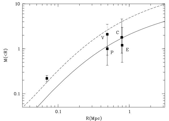
Fig. 3. Comparison of different mass estimates for XMMU J1007 in units of 10^{14} M_{\odot} . Labels indicate results based on scaling relations by Vikhlinin et al. (2009); Pratt et al. (2009); Carlberg et al. (1997); Evrard et al. (2008). The dashed and solid lines indicate universal density profiles (Navarro et al. 1997) with concentration parameters of 3.86 and 3.45 for virial masses 1.8 and 4.6 \times 10^{14} M_{\odot} at an assumed R_{vir} = 780 \text{ kpc} , respectively (Bullock et al. 2001).
