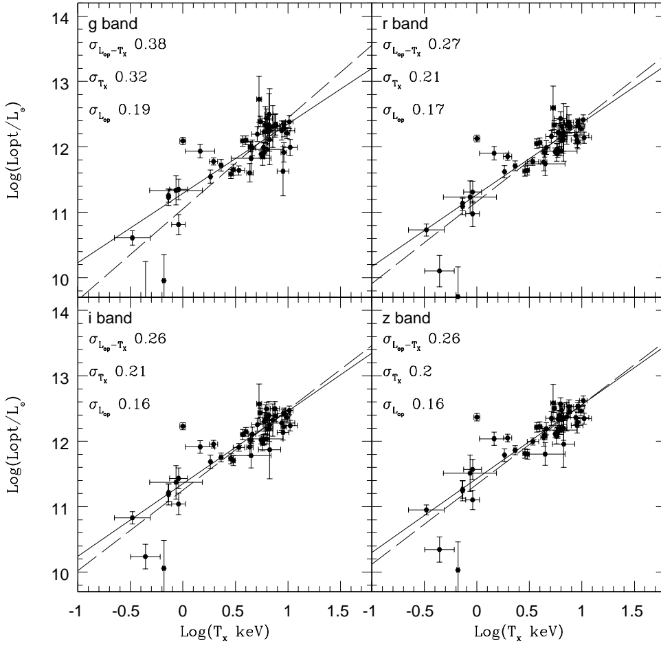
Fig. 19. Correlation between optical luminosities and ICM temperature. The fit is performed with a linear regression in the \log(L_{\text{opt}} - \log(T_x)) space for each of the 4 optical bands. The solid and the dashed lines are the results of the orthogonal and bisector method respectively. The error bars are at the 68% confidence level in both the variables.
